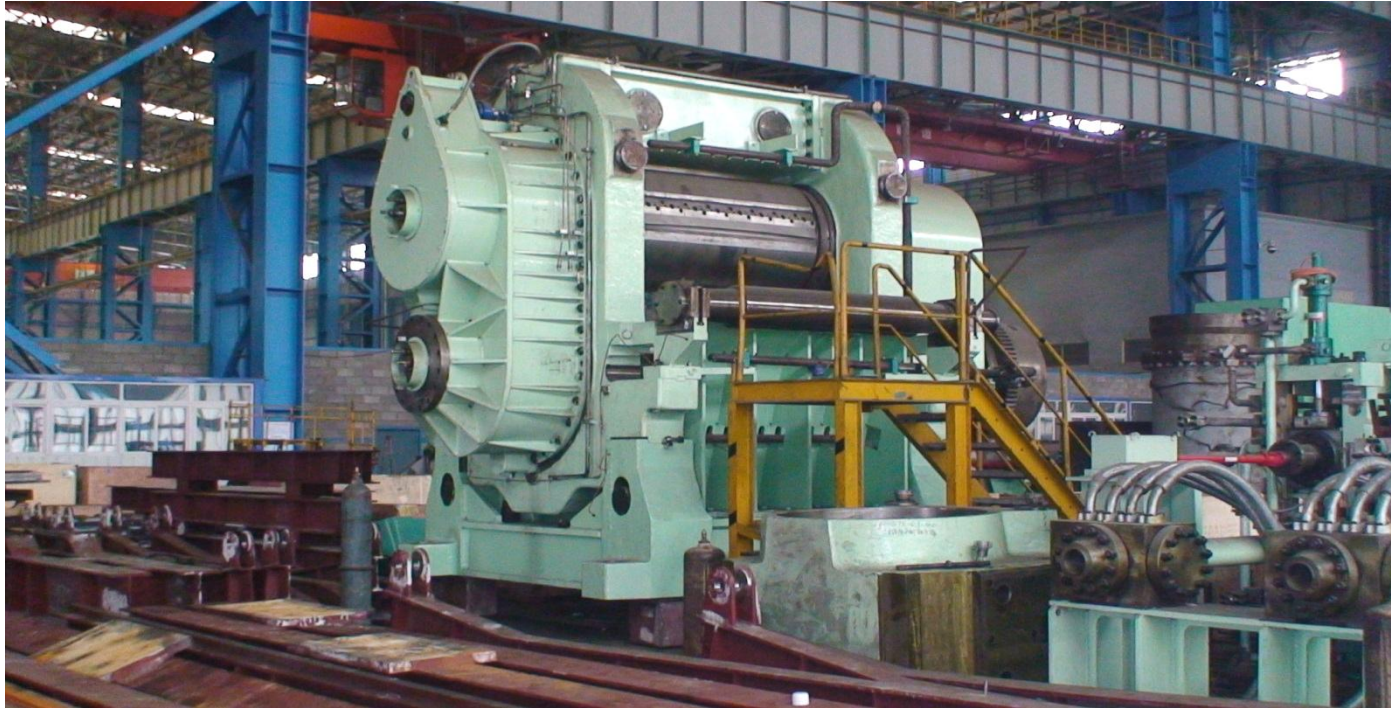
飞剪 Fly shear/Crop Shear
