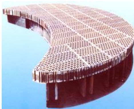
热风炉算子Checker Support System
